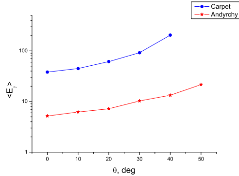
Figure 4: Average photon energy vs. zenith angle for model of [10].
