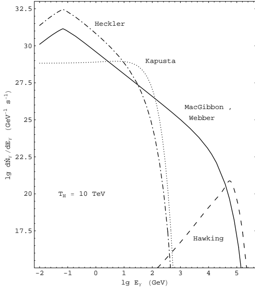
Figure 1: Instantaneous photon spectra from a black hole with Hawking temperature T_H = 10 TeV.
