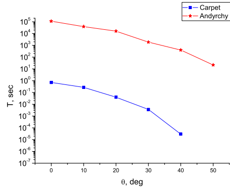
Figure 5: Time duration of gamma burst vs. zenith angle for model of [10].
