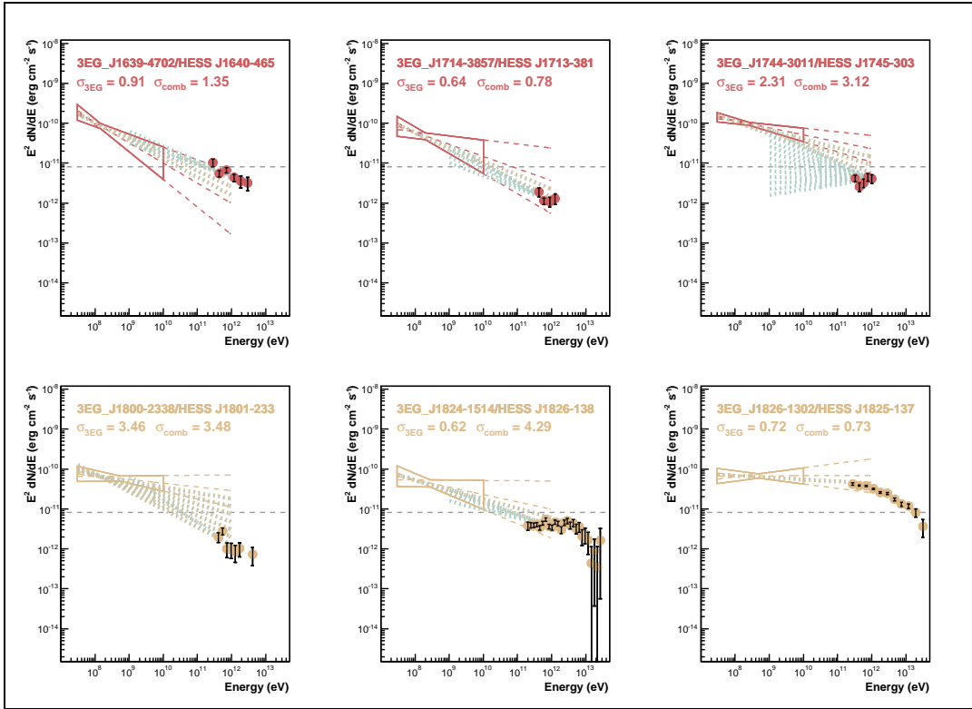
Figure 1: Spectra for the source in which a positional coincidence between EGRET and H.E.S.S. sources is given. The red plots show sources for which the H.E.S.S. source is located within the 95% confidence level whereas the orange plots show those within the 99% confidence contour (as give in Table 1)
