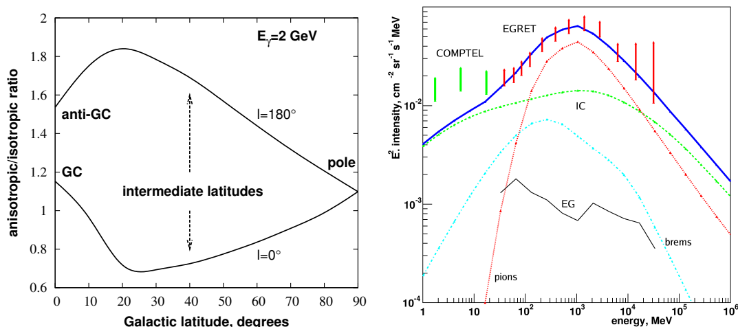
Figure 1: Left : The ratio of anisotropic IC to isotropic IC for Galactic longitudes l = 0^\circ and 180^\circ vs. Galactic latitude [9]. Right : \gamma -ray spectrum of inner Galaxy ( 330^\circ < l < 30^\circ , |b| < 5^\circ ) for the optimised model. Vertical bars: COMPTEL and EGRET data, heavy solid line: total calculated flux. This is an update of the spectrum shown in [7].
