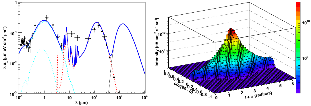
Figure 2: Left : Local ISRF spectral energy density. Line-styles: solid, total; thick dashed, stellar; thin dashed, scattered; chain, dust; dotted, CMB. Data points are summarised in [19]. Right : Model local ISRF intensity at 2.2 \mu\text{m} as a function of Galactic longitude l and latitude b .
