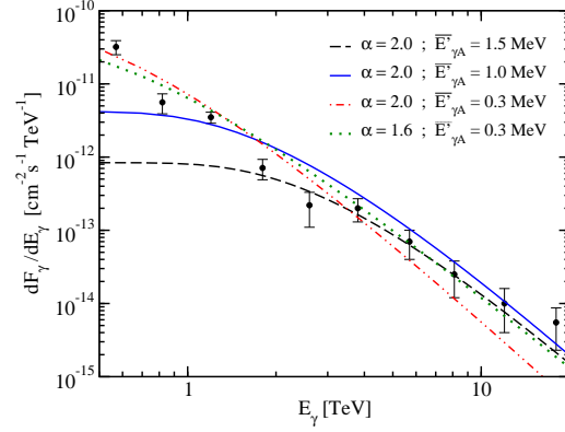
Figure 2: Sample eyeball fits to HESS Westerlund 2 \gamma -ray spectrum for the A^* model, with various values of the injection ^{56}\text{Fe} nuclei power index \alpha and the average energy E'_{\gamma A} of emitted de-excitation photons.
