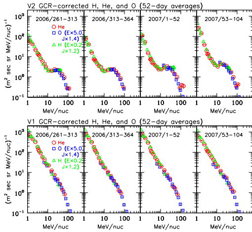
Figure 5: Same as Figures 3 and 4 except for the time periods.
