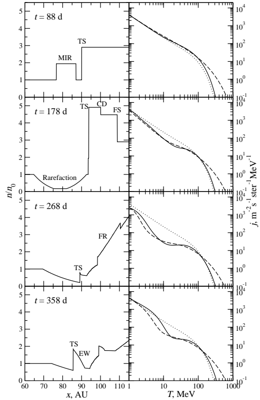
Figure 2: Model calculations of effect on energy spectrum of H of MIR interacting with termination shock (from [10]). Relative solar wind density is on the left and energy spectra are on the right. The dotted line shows the unperturbed original energy spectrum and the solid and dashed lines represent two different methods of modeling the MIR.
