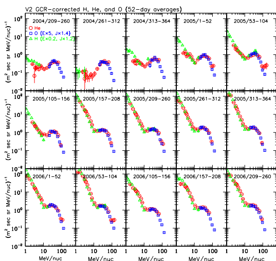
Figure 4: Same as Figure 3 except for V2.
