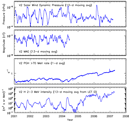
Figure 1: Voyager 2 observations of solar wind dynamic pressure, magnetic field magnitude, >70 MeV ion rate, and intensity of H with 2-3 MeV vs. time. Note the series of MIRs discussed in the text.
