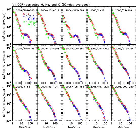
Figure 3: Energy spectra of H, He, and O at V1 for fifteen 52 day periods. The observed spectra have been corrected for galactic cosmic rays (GCRs) based on the observed C energy spectrum. V1 crossed the shock on day 351 of 2004. The H and O energy spectra have been scaled by factors in energy/nuc and intensity as shown in the figure.
