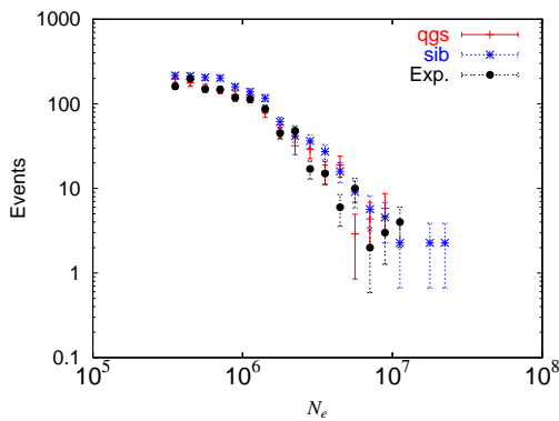
Figure 8: Burst triggered air-shower size spectrum
