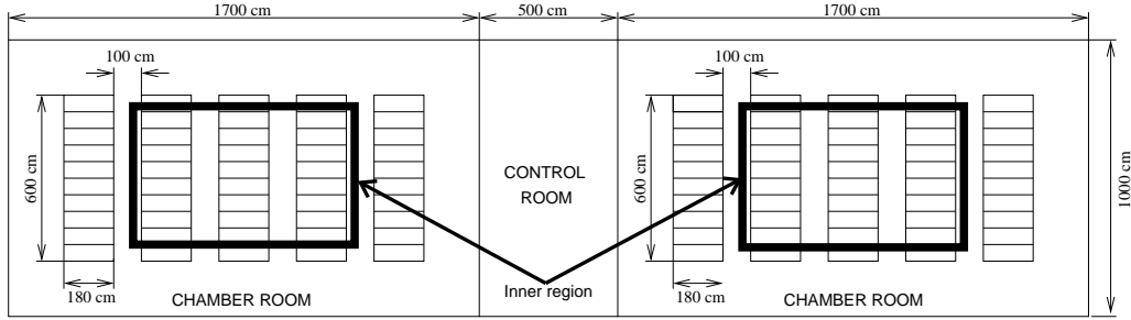
Figure 1: Arrangement of burst detectors
