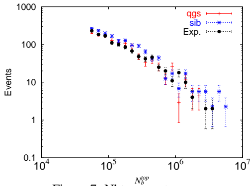
Figure 7: N_b^{top} spectrum
