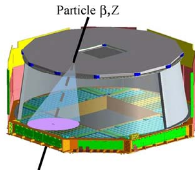
Figure 2: Schematic view of the RICH detector.
