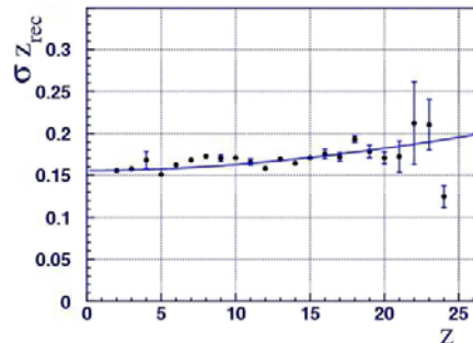
Figure 4: The RICH prototype charge resolution
