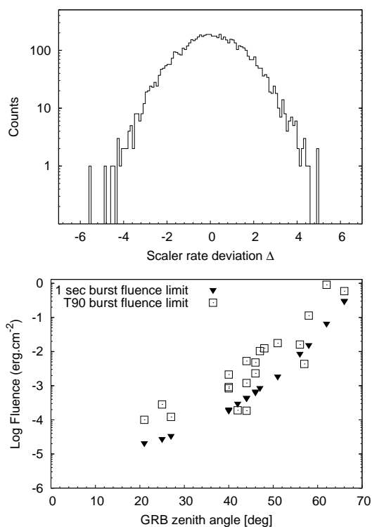
Figure 3: Top: histogram of the deviations \Delta of the scaler counting rates within 100 seconds of the bursts reported by satellites. No significant excess is observed. Bottom: 5\text{-}\sigma fluence limits in the 1 GeV - 1 TeV energy range from Auger for these bursts, for a single second burst or for a burst of duration T_{90} , assuming a spectral index of -2 .
