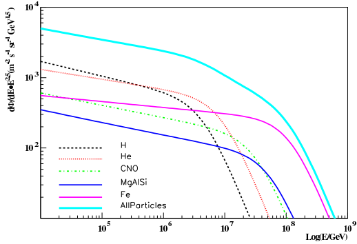
Figure 2: The fitted primary cosmic ray energy spectra according to [7].
