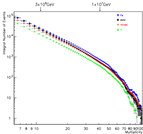
Figure 5: Integral distribution of the muon multiplicity measured in the single P-chamber. For comparison, the simulation results from both, the mixed and the single component model (i.e., pure proton and pure iron) are shown as well.
