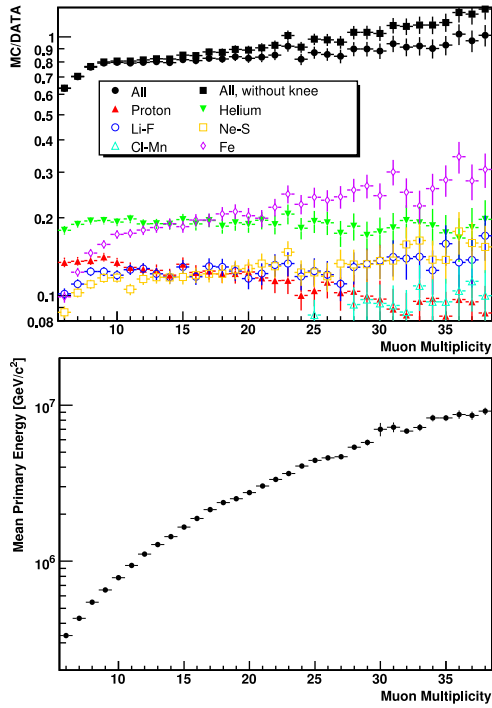
Figure 4: The muon multiplicity distribution ( N_\mu < 40 ) [8] measured by the 3 dimensional reconstruction program of L3+C. The corresponding energy range is also given in the bottom figure.
