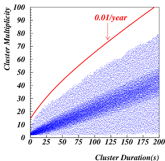
Figure 3: Clusters ( \Delta t, m ) detected during 2005-2007. The full line represents the LVD sensitivity in standalone mode ( F_{im} = 1 \cdot 10^{-2} \text{ y}^{-1} ).
