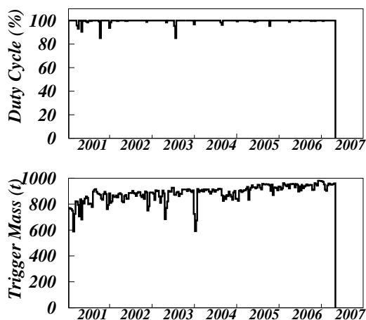
Figure 1: LVD duty cycle (top) and trigger mass (bottom) during years 2001-2007.
