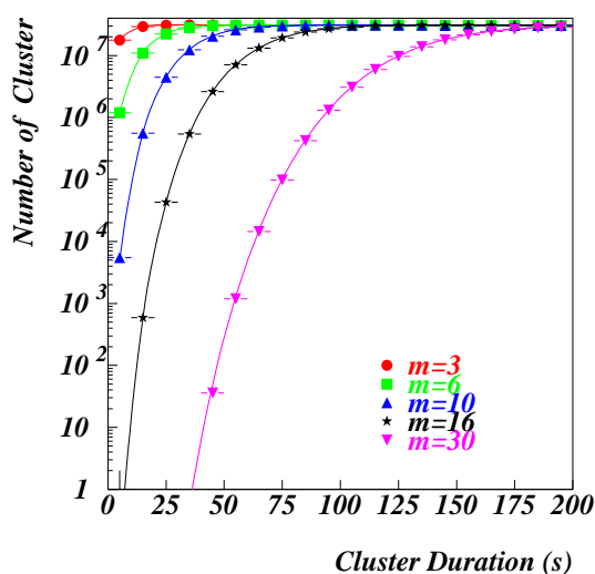
Figure 2: Distributions of the number of clusters, detected during 2005-2007, as a function of cluster duration ( \Delta t ), for different multiplicity ( m ).
