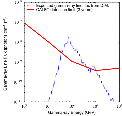
Figure 3: Gamma-ray line sensitivity of CALET for 3 years toward the Galactic center ( 300^\circ < \ell < 60^\circ , |b| < 10^\circ ), compared to the gamma-ray line flux from neutralino with the maximal annihilation rates [6] and Moore halo profile [4].
