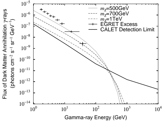
Figure 2: Diffuse and continuum sensitivity of dark matter annihilation gamma rays of CALET for 3 years, toward the Galactic center ( 300^\circ < \ell < 60^\circ , |b| < 10^\circ ), compared to the calculated continuum gamma rays from neutralino annihilation and an EGRET excess spectrum against the Galactic diffuse background gamma rays [7].
