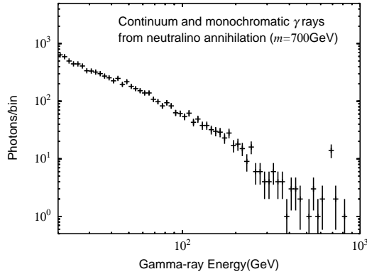
Figure 4: Simulated spectrum toward the Galactic center ( 300^\circ < \ell < 60^\circ , |b| < 10^\circ ) with CALET for continuum and monochromatic gamma rays from neutralino of 700 GeV mass with the Galactic diffuse background gamma rays.
