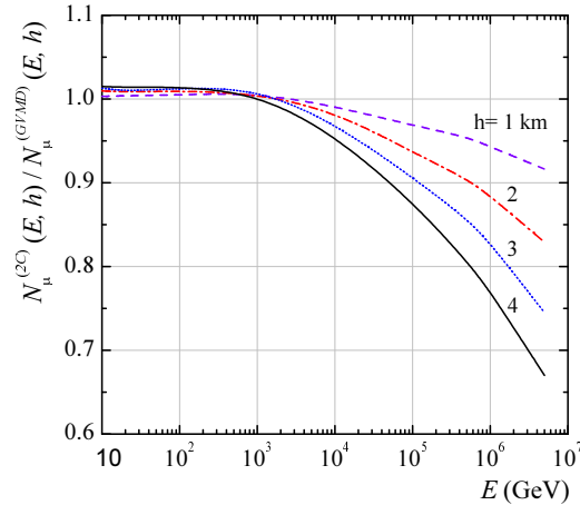
Figure 3: The ratio of muon fluxes underwater calculated with the 2C model to those obtained with the GVMD ones.
