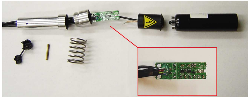
Figure 2: VERITAS pixel before assembly. The two-stage preamplifier is shielded in an aluminum shell. Two op-amps on the circuit board can be seen in the enlarged preamplifier image.
