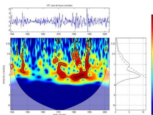
Figure 2: (a) High frequency time series of coronal hole area index b), c) And code color, same as figure 1
