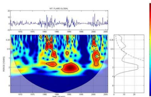
Figure 3: (a) High frequency time series of global flare index. b), c) and colour code, same as figure 1.
