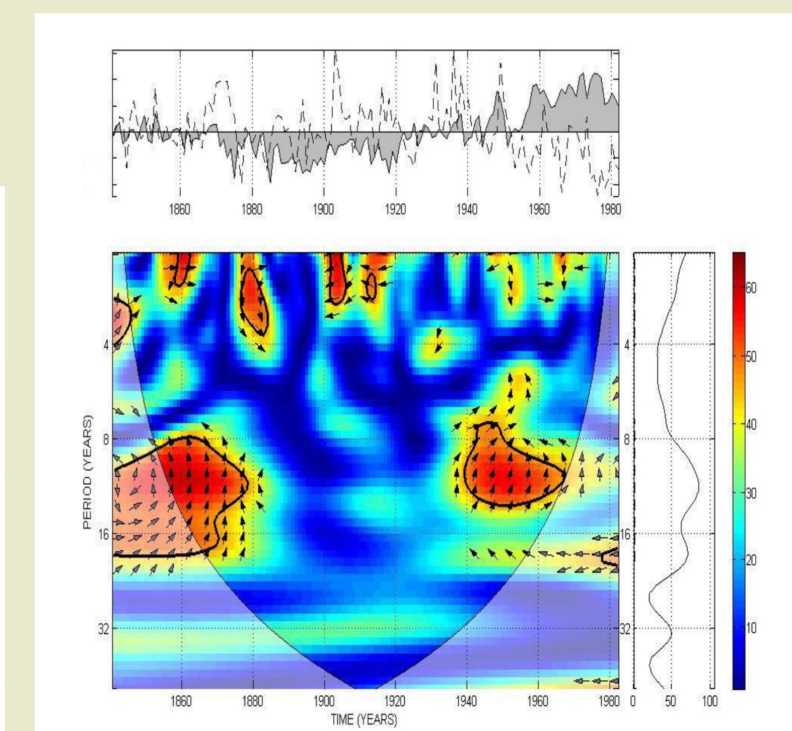
Figure 5. Wavelet and wavelet coherence analysis of Methane Sulphonic Acid (MSA) of high latitude north and Sea Surface Temperature (SST).
