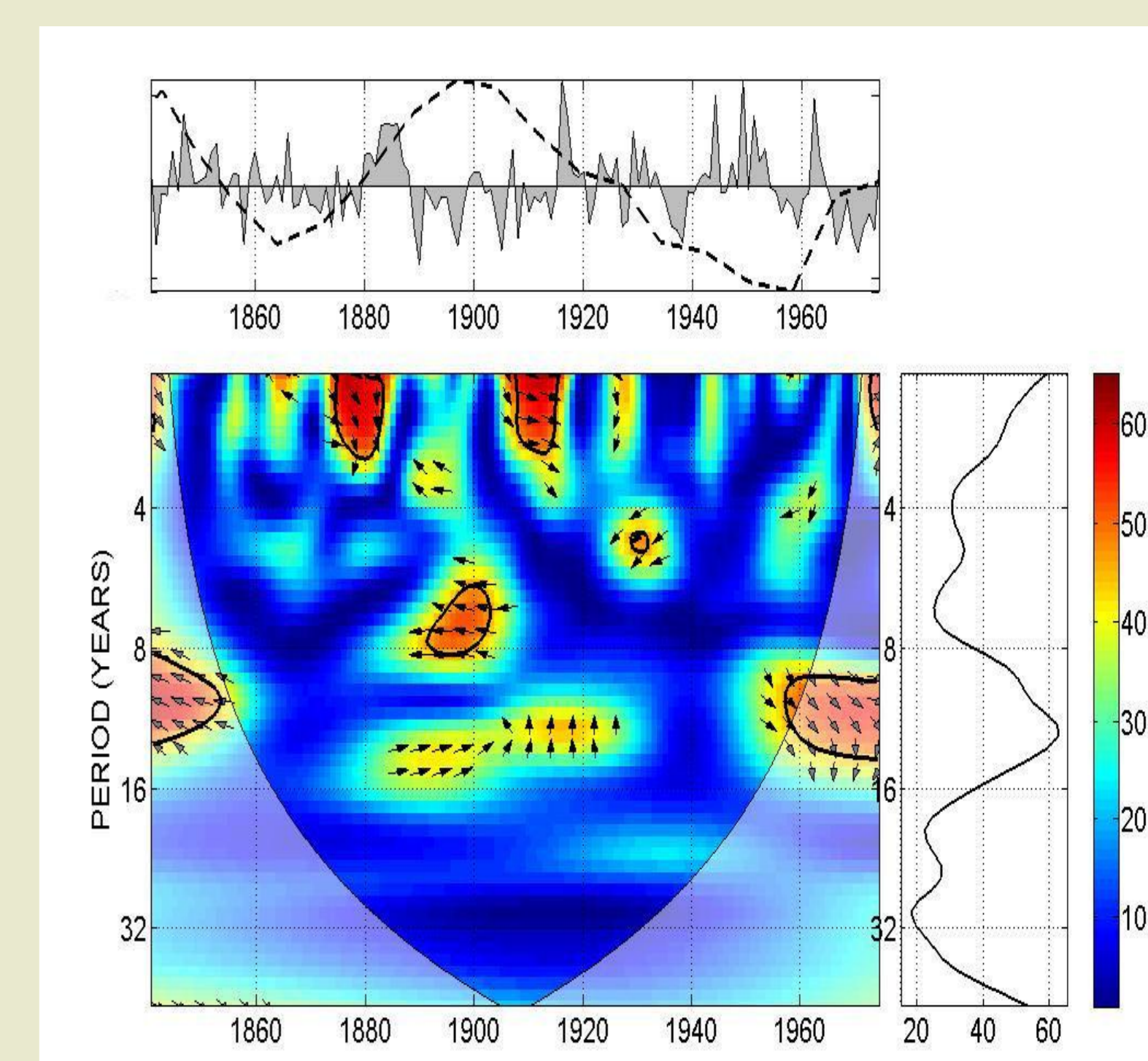
Figure 4. Wavelet and wavelet coherence analysis of Methane Sulphonic Acid (MSA) of high latitude south and Beryllium-10.
