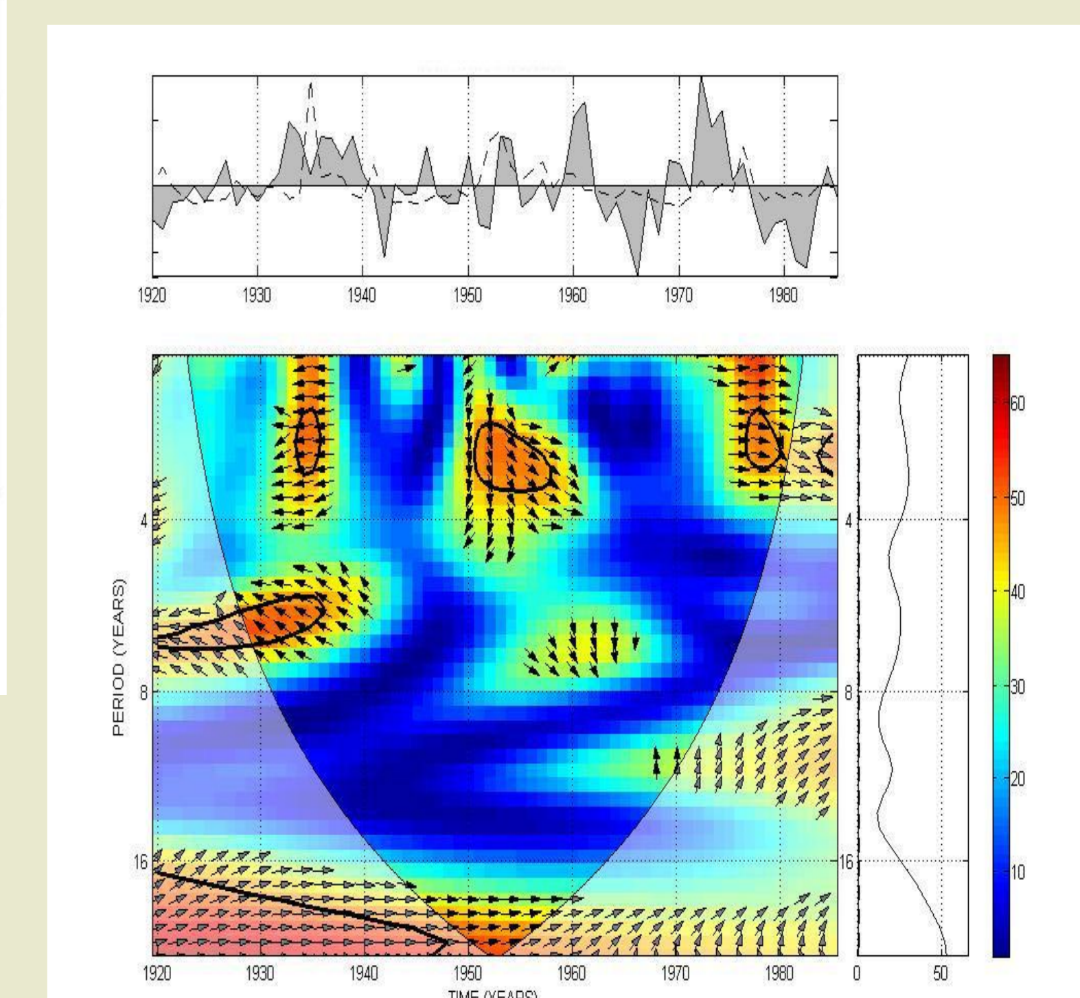
Figure 6. Wavelet and wavelet coherence analysis of Methane Sulphonic Acid (MSA) of high latitude south and Sea Surface Temperature (SST).
