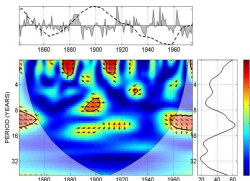
Figure 4: Wavelet and wavelet coherence analysis of Methane Sulphonic Acid (MSA) of high latitude south and Beryllium-10.
