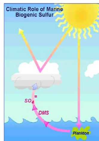
Figure 1: Hypothesized a climate feedback link where changes in cloud albedo and subsequent changes in surface temperature and/or solar radiation below clouds could affect the production of DMS by marine phytoplankton.
