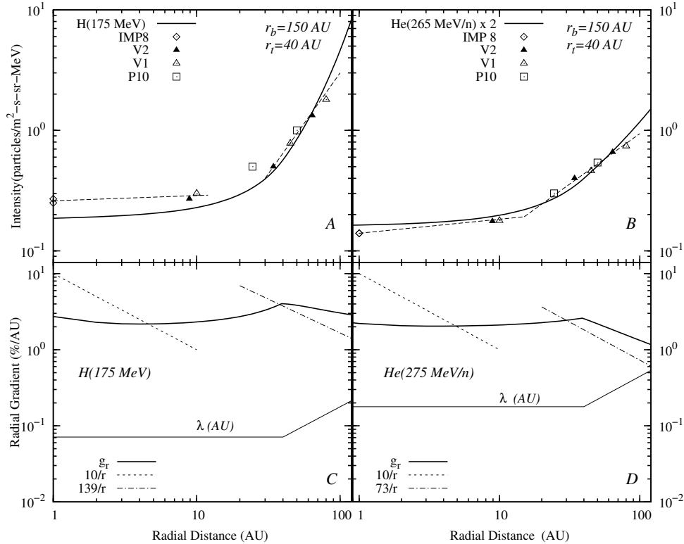
Figure 2: Radial intensity profiles (panel A for H and panel B for He) and radial gradient (panel C for H and panel D for He). Full lines are from a one dimensional model with a transition region at 40 AU and heliopause at 150 AU. Dashed, dotted and dash-dotted lines are from [6].
