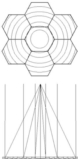
Figure 1: TUS mirror-concentrator.
