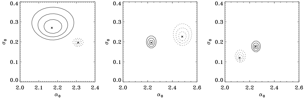
Figure 1: Left: Likelihood function 1\sigma , 2\sigma , and 3\sigma contours for the Mattox [3] (solid lines) and the 3EG [1] (dashed lines) confident blazar samples. Center: Same for BL Lacs (solid) and FSRQs (dashed). Right: Same for “mostly flaring” (solid) and “mostly quiescent” (dashed) blazars. The axes represent the mean ( \alpha_0 ) and spread ( \sigma_0 ) of the ISID. The maximum-likelihood parameters of each ISID are denoted by \times .
