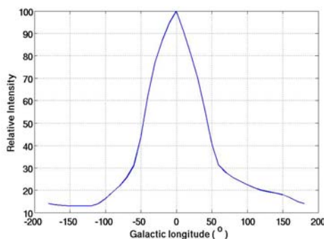
Figure 7: Radio signal intensity along the galactic plane [3].
