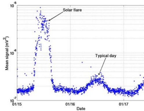
Figure 2: Mean squared signal over 10 \mu s vs time.
