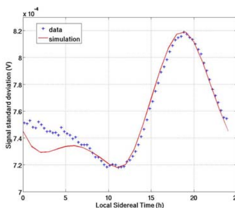
Figure 6: Averaged signal as a function of the local sidereal time over 6 months.
