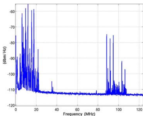
Figure 5: Frequency spectrum at Nançay.
