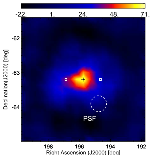
Figure 3: Preliminary smoothed morphology of gamma ray candidates from HESS J1303–631. The dashed circle of 0.^{\circ}23 is the point spread function. The empty squares indicate the tracking positions.
