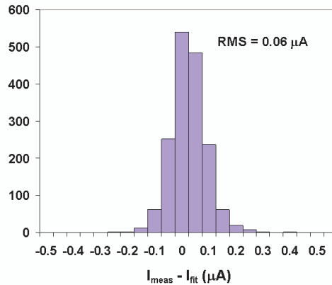
Figure 8: Distribution of the residuals of the RPC average current in cluster 91 with respect to the linear fit, based on the correlation plot in Fig. 7. The RMS is about 0.06 \mu\text{A} .
