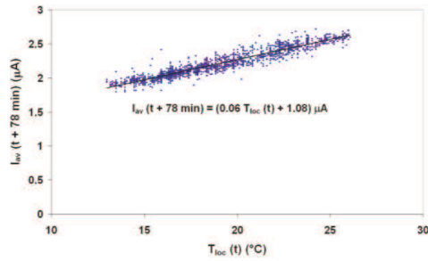
Figure 7: Correlation plot of the 78-minute delayed average RPC current and the local temperature for one ARGO-YBJ cluster near the carpet center (Cluster 91). The result of the linear fit is also shown.
