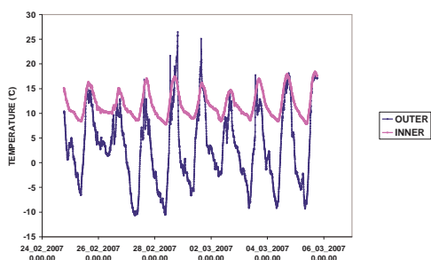
Figure 1: 8-day-long behaviours for the outer temperature and the inner temperature close to the RPC-carpet center, in February-March 2007.
