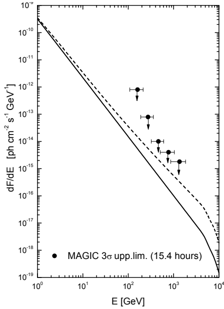
Figure 2: MAGIC upper limits to the differential \gamma ray flux of Arp 220. The curves represent the theoretical predictions: a solid line shows the result using the \delta -function ([21]) or Kamae ([22]) approximations for the proton-proton cross section, whereas a dashed line shows the result using the parameterization proposed by [23] extrapolated to high energies. Theoretical curves are from [8],[24]
