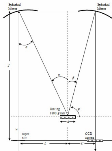
Figure 4: An optical configuration of the 1 m focal length spectrograph designed for recording the N 2 de-excitation UV light. The distances L , L' and w are geometrical design parameters, which have been appropriately selected for the UV range with a central wavelength of 350 nm.
