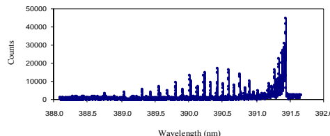
Figure 1: Spectrum of first negative band (around the line 391.44 nm), obtained experimentally by a 3 m focal length monochromator.
