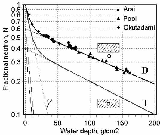
Figure 1: Curves of absorption of neutrons and gamma radiation: D for a detector located under snow and I located inside of snow. Experimental points show an absorption in snow at sea level (Arai и Pool) and in the mountain (Okutadami). Red curve shows an absorption of gamma. Data are adopted from [6].
