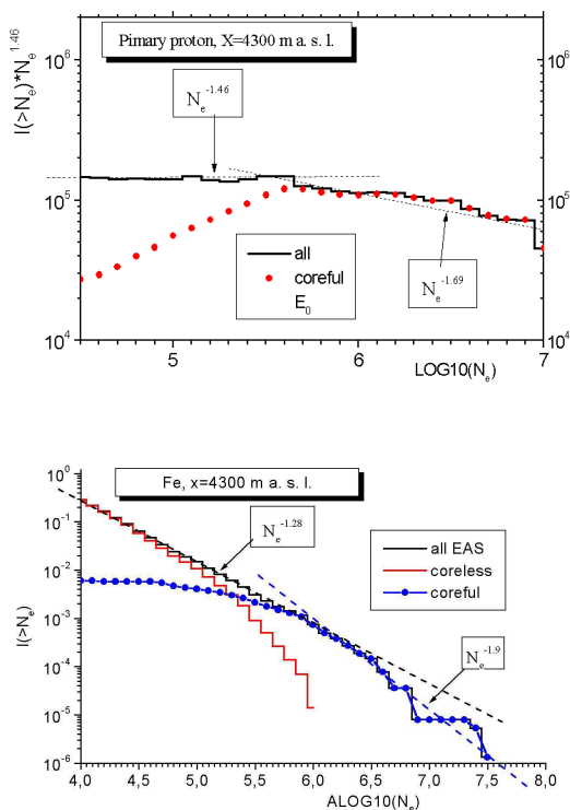
Figure 1: Results of Monte Carlo simulations for N_e distribution at 4300 m a. s. l. altitude. Top panel for protons (multiplied by N_e^{1.46} ), low panel for iron nuclei.
