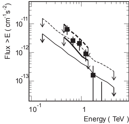
Figure 2: Upper limits on the gamma-ray flux from NGC 253 [13]. The points with error bars are the CANGAROO-II fluxes [10, 11]. The thin solid line is 99% upper limit (UL) by H.E.S.S. for point source assumption, and the thin dashed is that for 0.5 degree diffuse source [12]. The thick solid line is 2\sigma upper limit for this observation for point source assumption and the thick dashed line for 0.5 degree diffuse.
