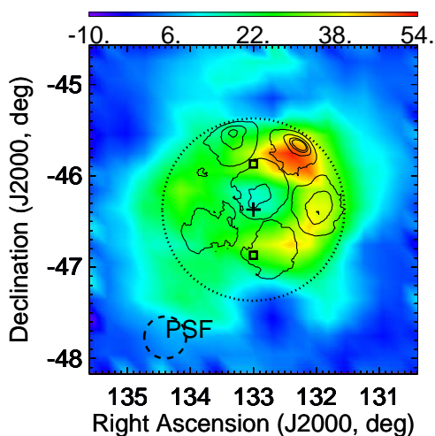
Figure 1: Excess event map around the SNR RX J0852.0-4622 obtained from the CANGAROO-III stereo observations in 2005 [7]. The vertical scale (number of events per pixel, 0.2^\circ \times 0.2^\circ ) is indicated in the top bar. The cross indicates the average pointing position, i.e., the center of the remnant and the squares the “wobble” pointing positions. The dashed circle of 0.23^\circ shows the ( 1\sigma ) point spread function. The dotted circle of 1 degree from the supernova center is also shown. Overlaid contours show X-ray intensity observed by ASCA GIS.
