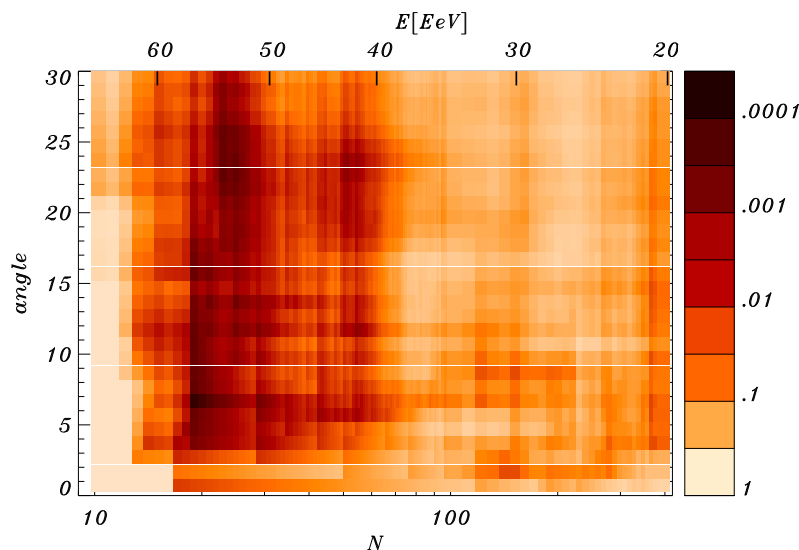
Figure 2: Autocorrelation scan for events with energy above 20 EeV
