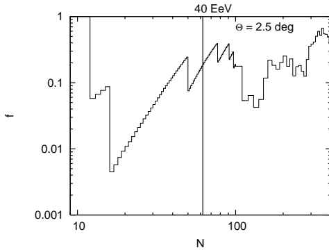
Figure 4: Fraction of simulations with more pairs separated by \theta < 2.5^\circ , as a function of the number of events.
