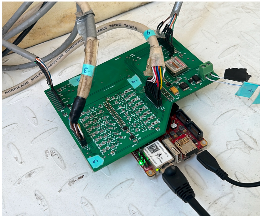
Pitaya Network (red board) connecting with drivers board (green board).
