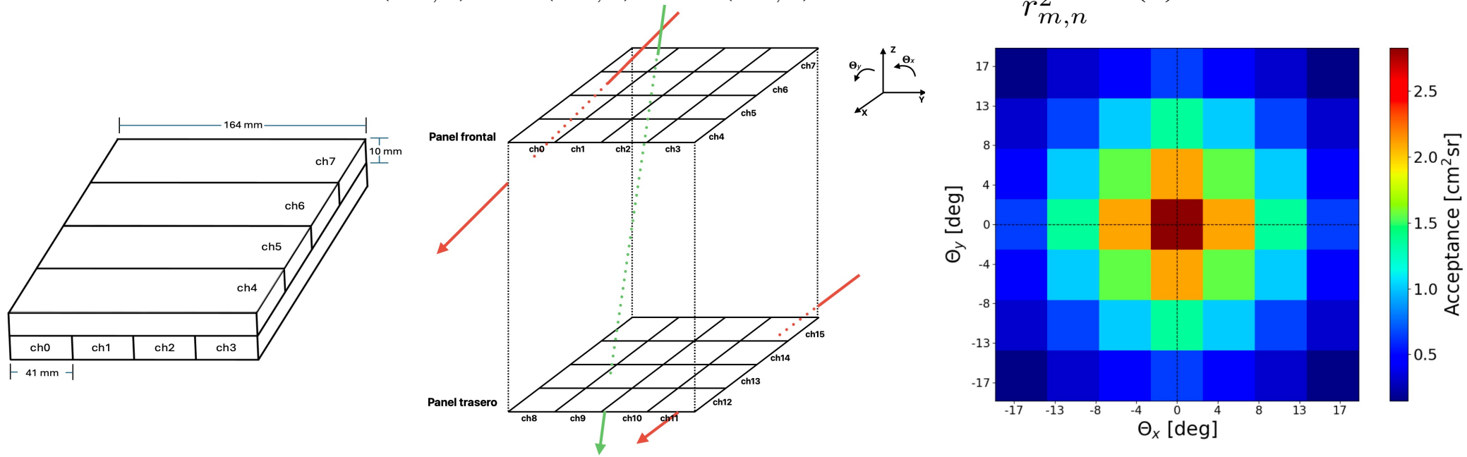
Arrangement of the detector channels (left) and their geometric acceptance (right).
