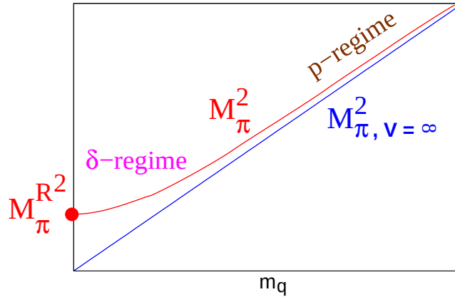
Figure 2. A qualitative picture of the expected behaviour of the pion mass squared in a \delta -box. For heavy quarks and pions we approximate the p -regime relation m_q \propto M_\pi^2 . For light quarks the pion mass attains a plateau, and finally (in the chiral limit m_q = 0 ) the residual value M_\pi^R .
