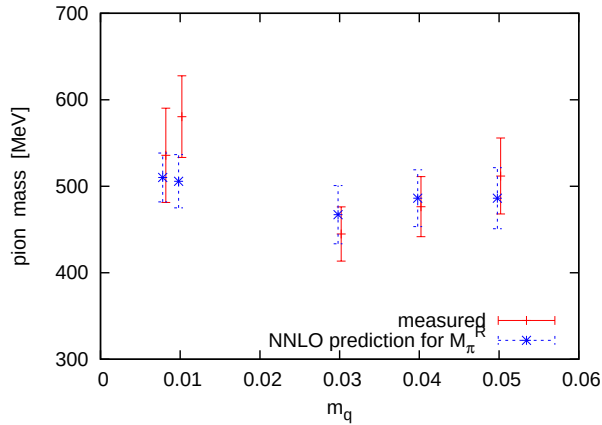
Figure 3. An illustration of our results given in Table 1: we show the numerically measured pion mass and the theoretical residual mass M_\pi^R , as predicted by the NNLO \delta -expansion. (The latter actually refer to the chiral limit, but its value depends on L and therefore on the lattice spacing a , which varies for the simulations at different m_q .) We observe a decent agreement between the measured and the predicted values.
