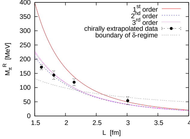
Figure 6. A comparison of our extrapolated values for the residual pion mass M_\pi^R with the predictions by the \delta -expansion, as functions of the spatial box size L . We observe a remarkably good agreement. In our largest volume, the extrapolated M_\pi^R is located below the physical pion mass, and in the region M_\pi^R L < 1 , which can be viewed as the domain of the \delta -regime.
