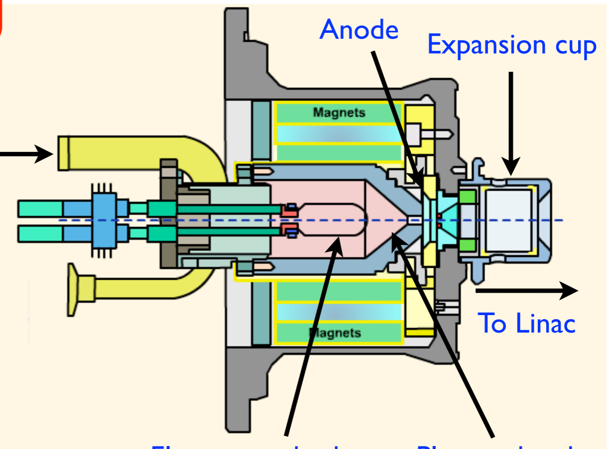
Electron cathode
