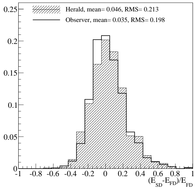
Figure 2: Energy resolution.
