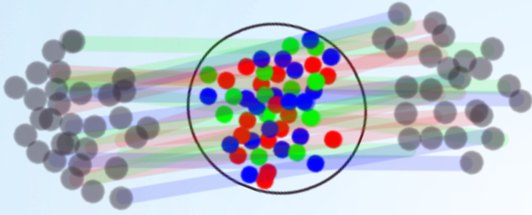
Shear Viscosity
