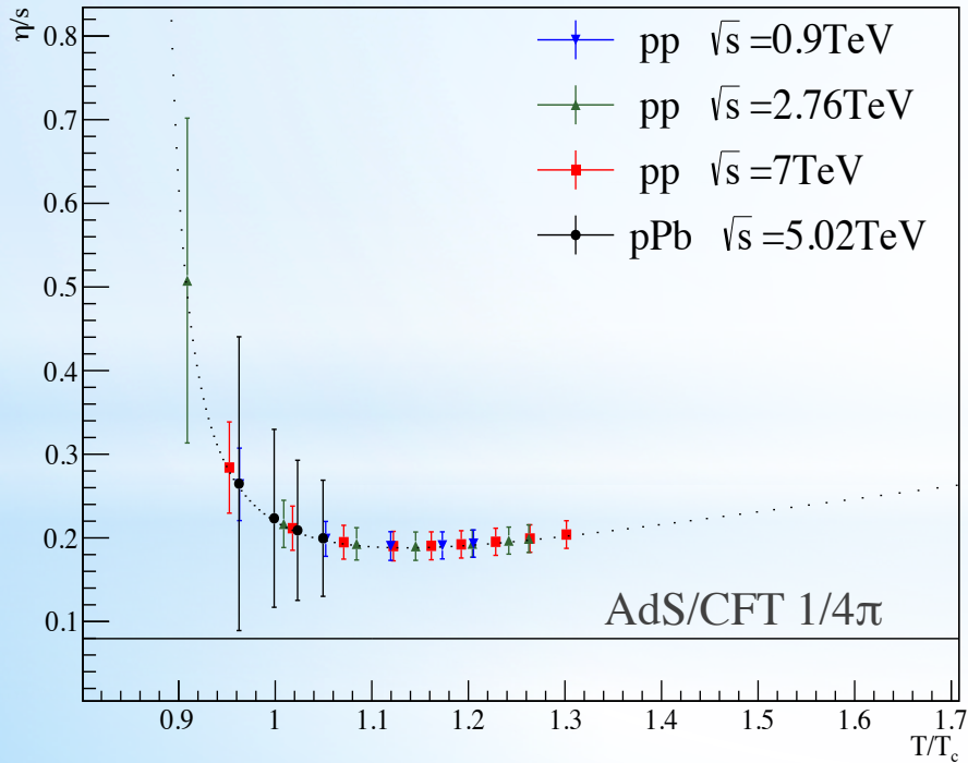
Shear Viscosity
