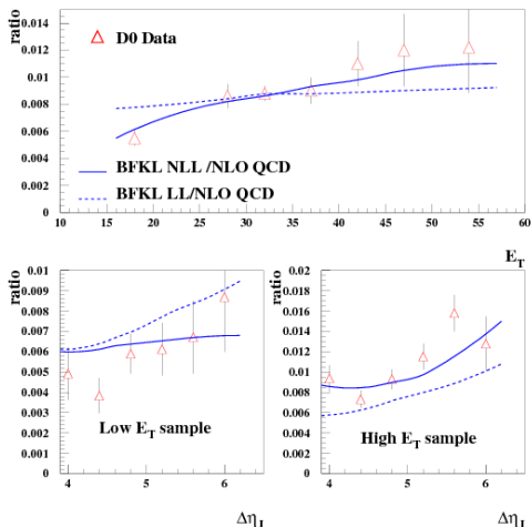
Figure 6. Comparisons between the D0 measurements of the jet-gap-jet event ratio using the NLL-BFKL kernel (solid line), LL-BFKL (dashed line) predictions with respect to the 2-to-2 NLO DGLAP prediction. Taken from [36]. The NLL calculation is in fair agreement with the data while the LL one leads to a worse description.
