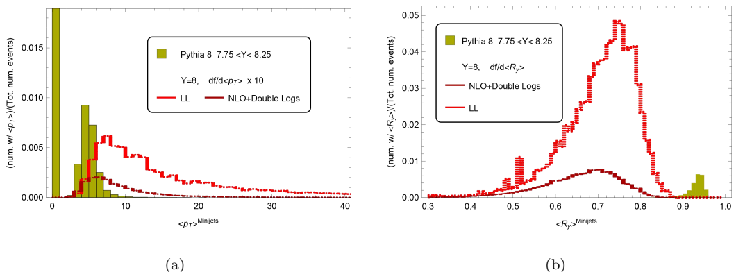
Figure 4. Preliminary comparison of mini-jet p_T and R_y between BFKLex (red curves) and DGLAP-based PYTHIA8 (gold). PYTHIA results have been rescaled by one order of magnitude for ease of comparison. BFKLex data is from [20].
