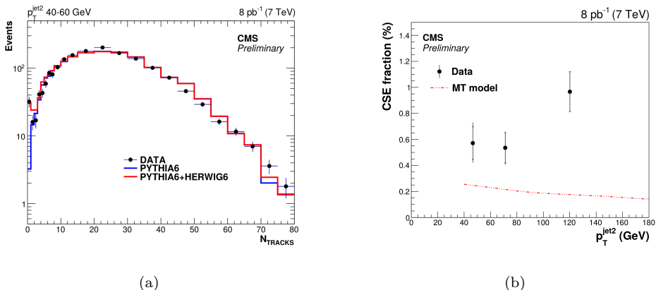
Figure 7. From [39]: (a) Number of charged particle tracks N_{\text{Tracks}} for 40 \text{ GeV} < p_T^{\text{sublead}} < 60 \text{ GeV} with |\eta^{1,2}| > 1.5 and \eta^1 \cdot \eta^2 < 0 in the fixed rapidity interval |\eta| < 1 of CMS. The red curve combines the LL M-T dijet and PYTHIA6 NLO dijet events. The excess at low multiplicities can be explained due to the color-singlet exchange. (b) The fraction of color-singlet exchange f_{\text{CSE}} dijet events as a function of the subleading p_T measured for \sqrt{s}=7 \text{ TeV} , compared to the LL BFKL predictions for N_{\text{Tracks}} = 0 . A large numeric and qualitative disagreement between the two can be seen.
