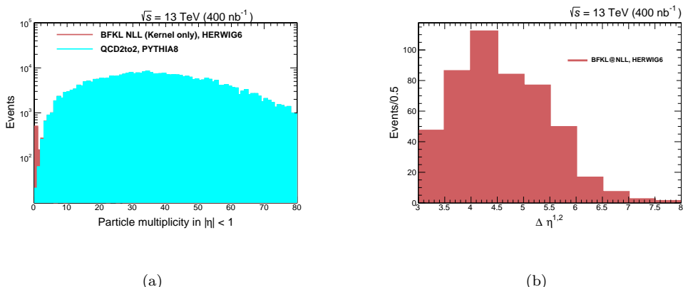
Figure 8. (a) Particle multiplicity in the fixed rapidity region |\eta| < 1 . Stable particles pass the selection cut p_T > 0.2 GeV. A high-purity Mueller-Tang dijets sample can be extracted in the lowest multiplicity bin. (b) Rapidity separation between the two hardest jets in the lowest multiplicity bin.
