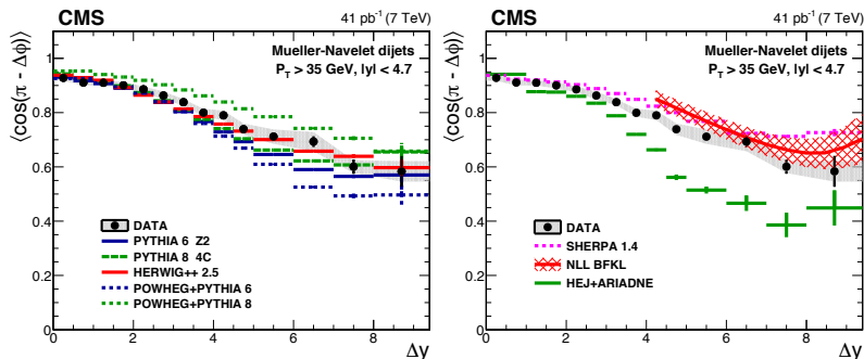
Figure 3. From [12], average \cos(\Delta\phi) , i.e. C_1/C_0 , as a function of the rapidity difference Y compared to DGLAP MC generators on the left and to the analytic NLL BFKL calculations at partonic level on the right. Similar analysis holds for most other ratios C_m/C_n .
