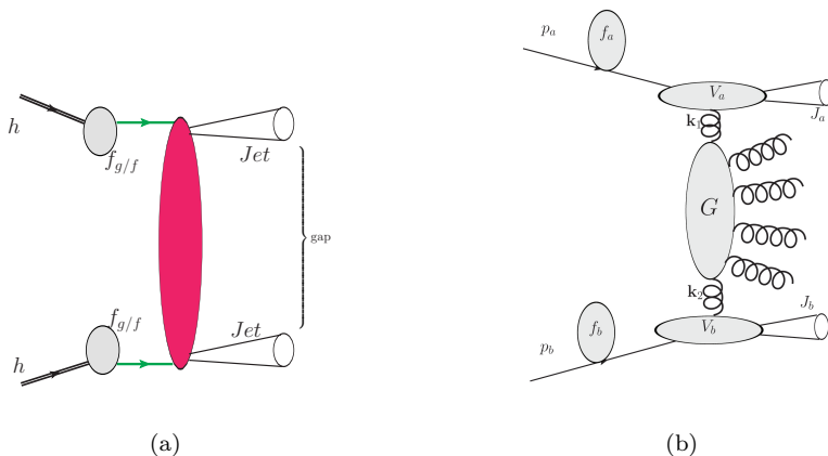
Figure 2. (a) Mueller-Tang jet-gap-jet process. (b) Mueller-Navelet inclusive dijet process.
