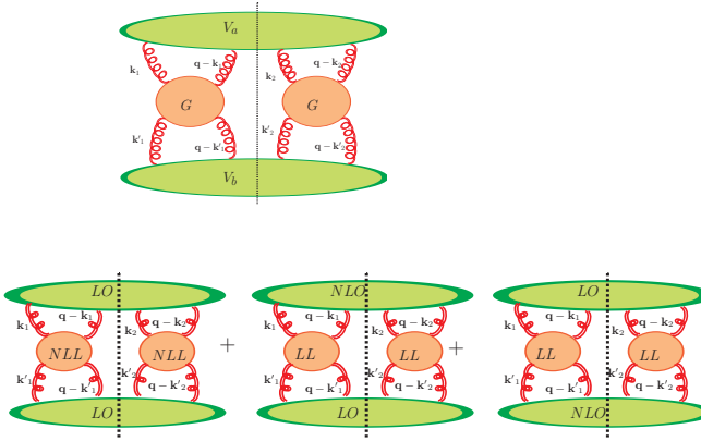
Figure 5. (Top) Schematic representation of the partonic elastic scattering via color-singlet exchange. G denotes the Green function and V the impact factors. (Bottom) Combinations of jet vertex and Green's function order that contribute to the full NLO M-T process.
