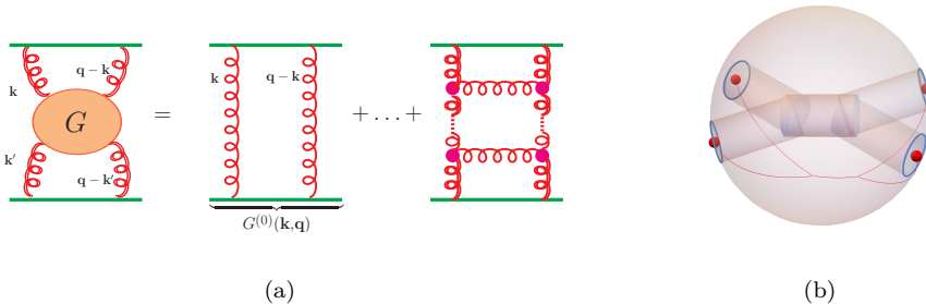
Figure 1. (a) Ladder diagram for the BFKL weak coupling Pomeron. (b) Cartoon of a 2-to-2 scattering process using the AdS/CFT applicable for the BPST strong coupling Pomeron.
