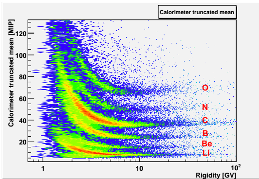
Figure 5: The ionization loss in the calorimeter with truncated mean using three points and at least four dE/dx measurements versus rigidity. A rough cut was used to throw away Helium nuclei which appear as a diffused region at about 2 GV and 5/6 MIP energy release.
