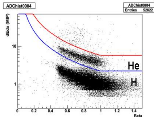
Figure 1: The ionization loss in a S12 scintillation counter vs. Beta. The solid curves show the selection criteria for Z=2 and Z>2 particles.
