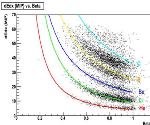
Figure 2: Charge separation obtained with one of the S12 scintillator, illustrated by plotting the ionization energy loss vs. the particle velocity. The solid curves show the theoretical behavior.
