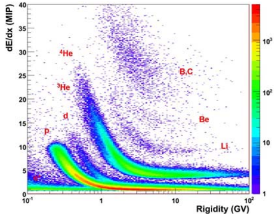
Figure 3: The ionization loss in the tracker vs. rigidity.
