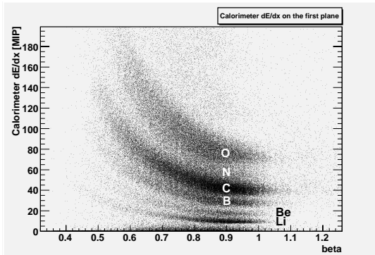
Figure 4: The ionization loss in the first plane of the calorimeter vs. the particle velocity.
