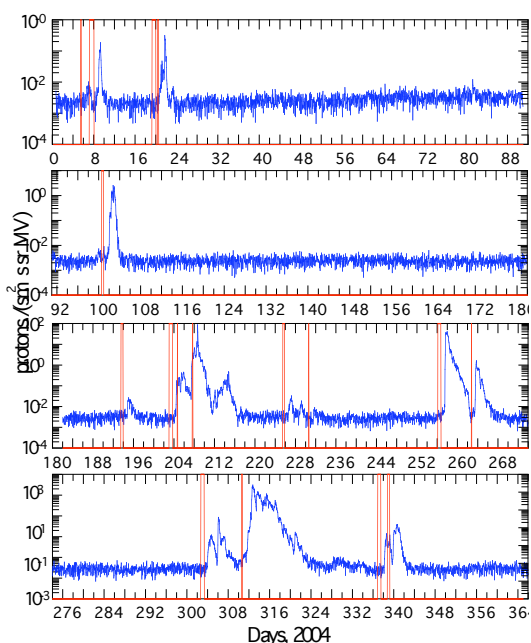
Figure 2: Time profile of CR intensity in energetic range 4–9 MeV in 2004. Moments of SPE predictors' appearance are shown by vertical lines.
