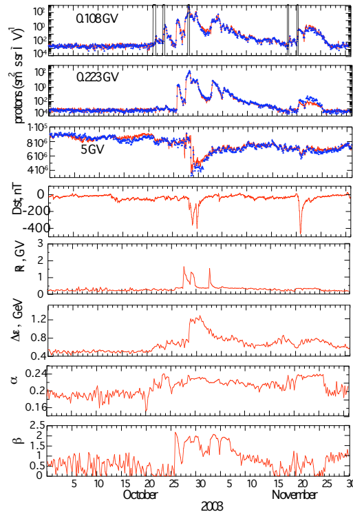
Figure 1: Temporal profiles of CR intensity with R=0.108, 0.223 and 5 GV (bold line – calculation, triangles – observations data), Dst-index and parameters of CR rigidity spectrum R_0 , \Delta\epsilon_1 , \alpha , \beta for the period October – November, 2003. Moments of SPE predictors’ manifestation are marked by the vertical lines at the upper panel.
