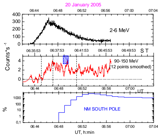
Figure1: Gamma emission time profiles observed by the SONG (upper panels) and GLE measured by South Pole NM (lower panel). The time scale between the first and second panels represents solar time of the event.
