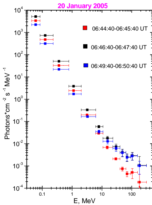
Figure2: The photon spectra measured by SONG.
