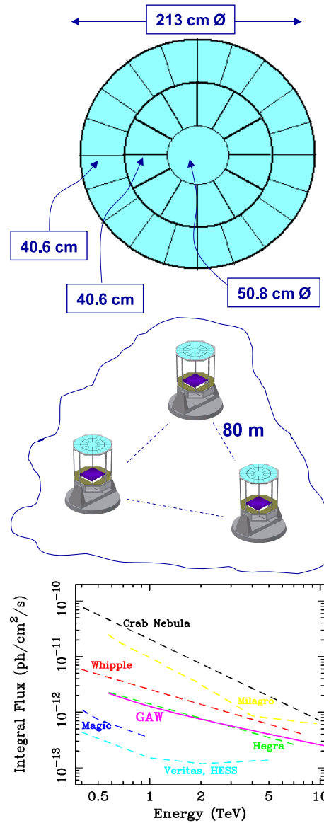
Fig. 3. Top: Fresnel lens design for GAW. Middle: Layout of the GAW 3-telescope array Bottom: GAW phase-II flux sensitivity ( 5\sigma in 50 h). Plots are taken from [30].
