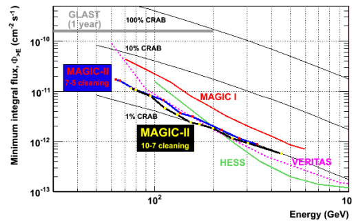
Fig. 2. Top: Variation of MAGIC energy threshold vs. pixel discriminator threshold (DT) and Moon phase [21]. Middle: Picture of the two MAGIC telescopes – MAGIC-II [18]. Bottom: MAGIC-II flux sensitivity (for two versions of image cleaning) compared with that from other \gamma -ray telescopes [18].
