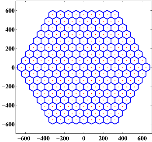
Fig. 7. Array layout for 217 \times 10 m diameter telescopes with 80 m spacing [47].
