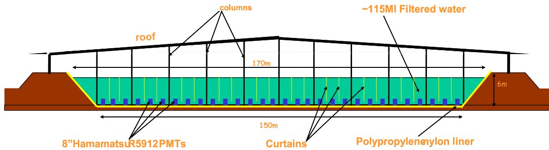
Fig. 11. HAWC schematic indicating location of PMTs and isolation curtains [57].
