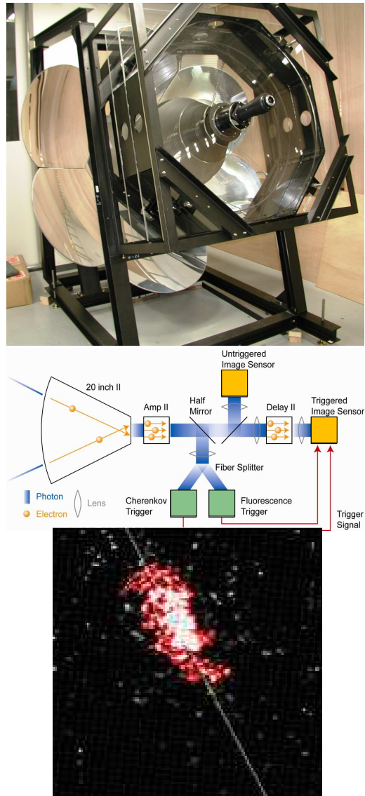
Fig. 4. Top: Modified Baker-Nunn optic of an ASHRA telescope. Middle: Detector and data flow for the various types of signal (optical, Cherenkov, fluorescence). Bottom: Example Cherenkov image. All images from [32].
