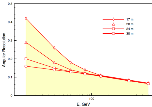
Fig. 9. Angular resolution for a three telescope system vs. telescope diameter [50] (telescope separation is 50 m).
