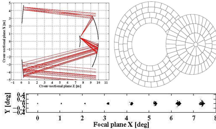
Fig. 8. Upper left: Off axis ray tracing for the Schwarzschild-Couder (SC) outlined by [47, 48]. Upper right: Segmented primary and secondary mirror layouts. Bottom: Off-axis focusing of a particular SC design.
