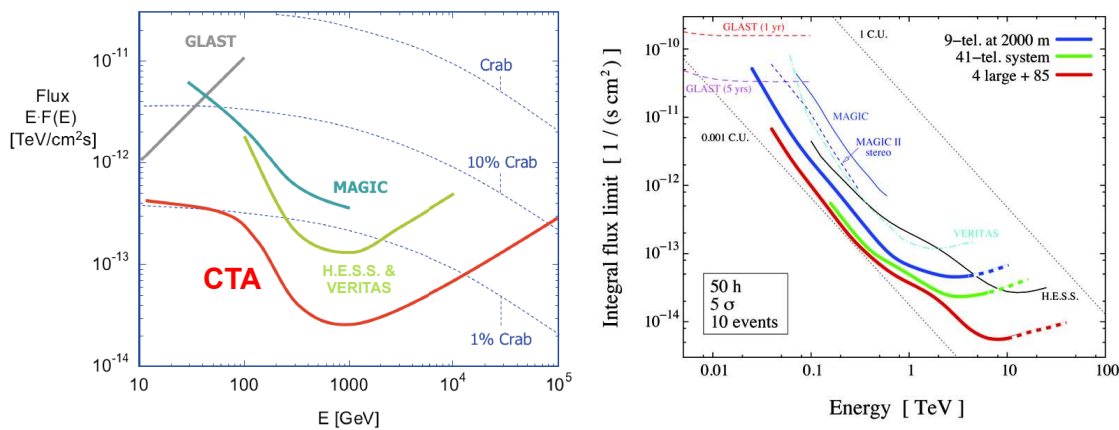
Fig. 6. Left: Desired flux sensitivity of CTA. Right Integral flux sensitivities for several telescope combinations considered in CTA simulations so far – 9-tel (group 1), 41-tel (group 2), 85+4-tel (group 3). See text for explanations of telescope groups. Figures are from [41, 44].
