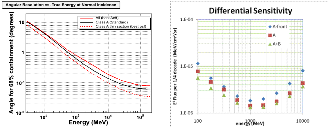
Fig. 5. Left: GLAST LAT angular resolution vs. energy. Right GLAST LAT flux sensitivity for one year observation. Figures are from [37].
