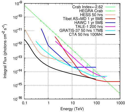
Fig. 13. Integral flux sensitivity of the proposed Tibet AS + muon detector (MD) array after 1 yr observation (red line).
