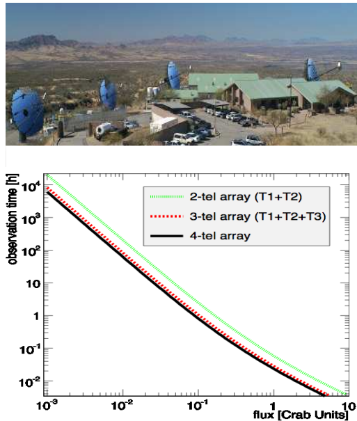
Fig. 1. Top: View of the VERITAS 4-telescope IACT array [4]; Bottom: VERITAS flux sensitivity (Crab units) of the VERITAS array for several telescope (T1, T2, etc..) combinations [16].
