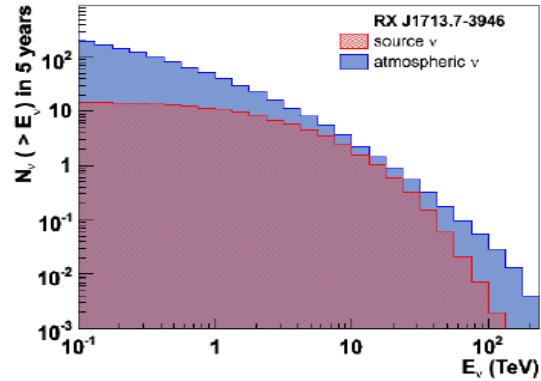
Fig. 15. Neutrino event count (in 5 yr) predicted from RX J1713–3946 (source \nu ) and atmospheric neutrino count vs. energy [65].
