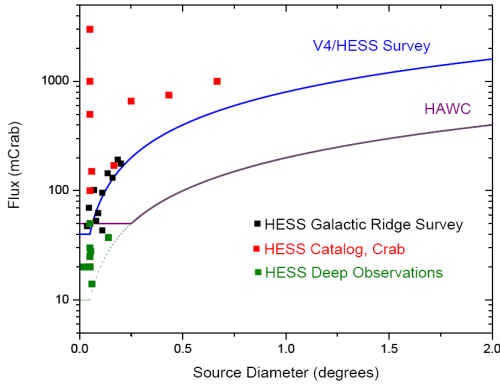
Fig. 12. Two year survey sensitivity of HAWC in comparison with several H.E.S.S. surveys. [57]
