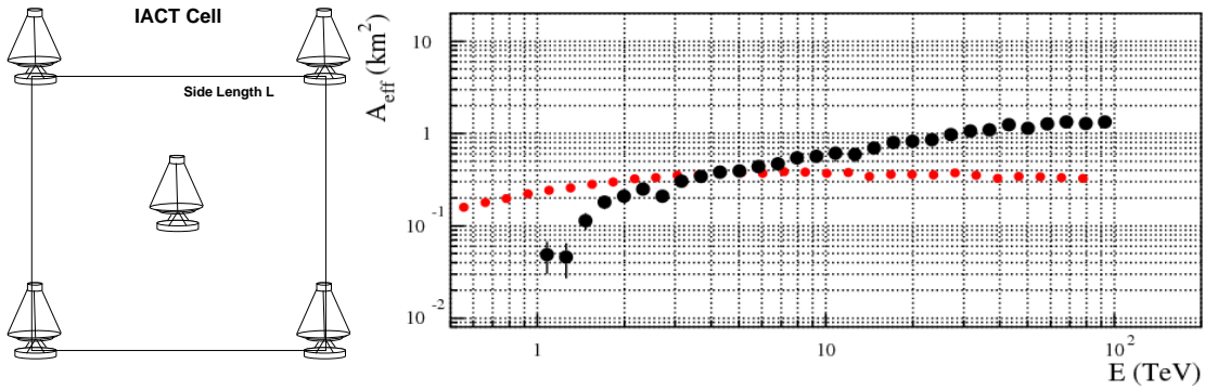
Fig. 10. Left: Layout of an IACT cell of 5 telescopes as simulated for TenTen . Results for L = 300 m were presented. Right: Effective area A_{\text{eff}} ( \text{km}^2 ) vs energy E (TeV) for the 5-telescope cell of side length L=300 m, at 200 m a.s.l. (large black solid circles). The effective area achieved by H.E.S.S. is shown as small red solid circles. In both cases, no selection cuts on \gamma -ray events are applied.
