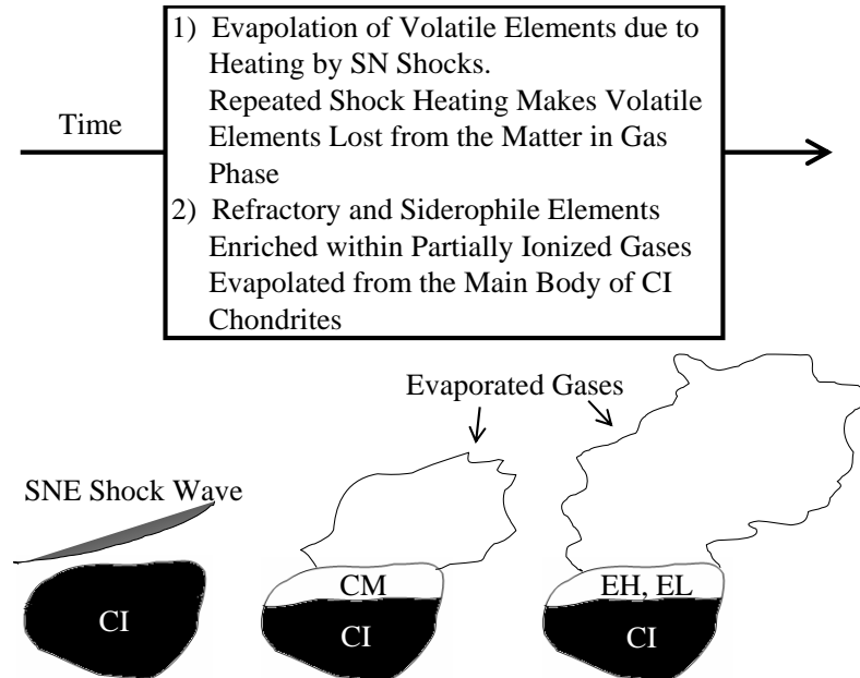
Figure 3: A possible time sequence for the source composition of galactic cosmic rays to be formed as the result of the interaction of dust grains with SNE shock waves in the interstellar space (Sears, 2004).
