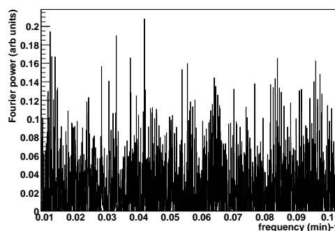
Figure 4: [ 10^{-2} \text{ min}^{-1} - 0.1 \text{ min}^{-1} ] Lomb-Scargle periodogram of the H.E.S.S. SgrA* light curve averaged over the 2004-2006 nights of observation. No significant peak is visible.
