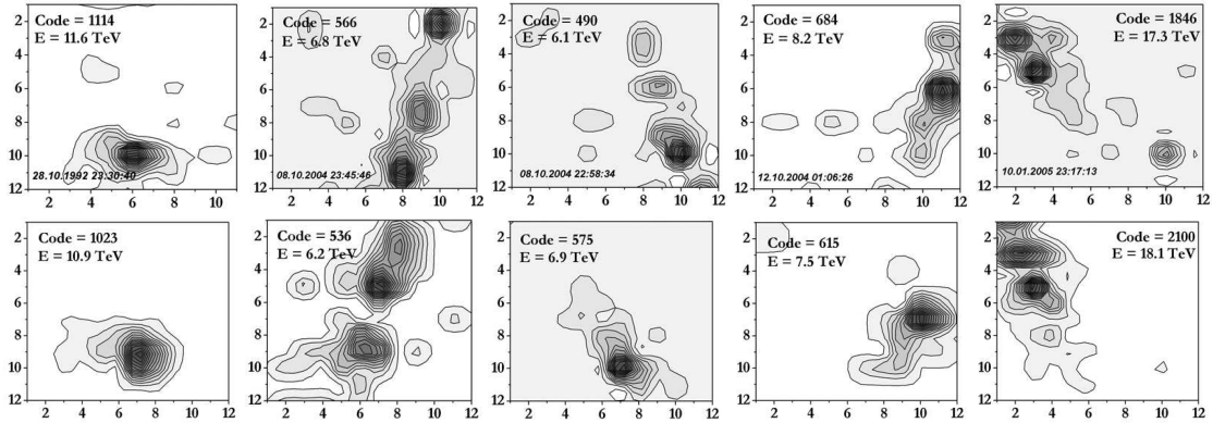
Figure 5: top - Cherenkov Radiation of Extensive Air Showers Observed at 97^\circ Zenith Angles by SHALON; bottom - Cherenkov Radiation of Extensive Air Showers Observed at 0^\circ Zenith Angles by SHALON.
