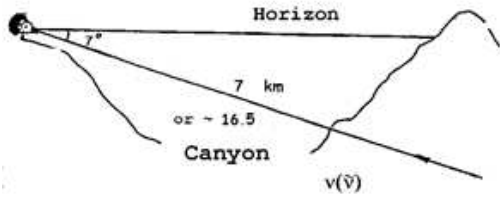
Figure 2: The geometry of down horizontal observation sessions.
