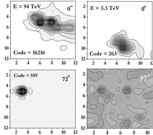
Figure 4: The examples of showers recorded in PMT matrix at different zenith angles. The amplitude of gray - scale shower images is proportional to the ADC count. The number, named CODE shows the range of detected signals in the ADC counts, which are proportional to shower energy.
