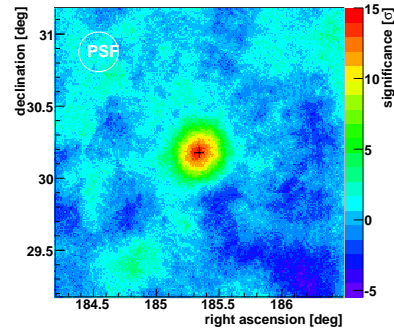
Figure 5: Significance map of the region around 1ES 1218 +304.
