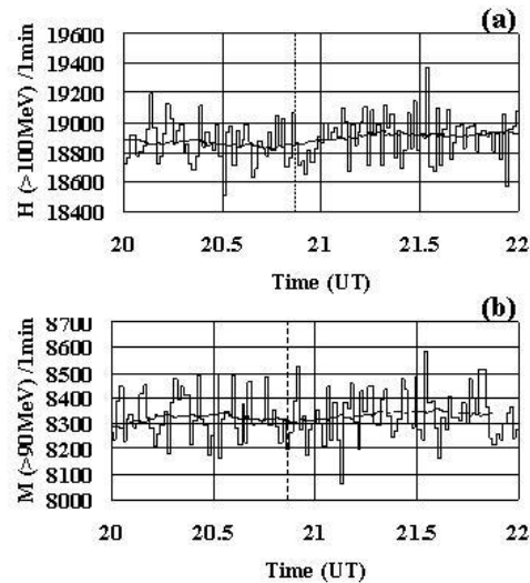
Figure 3: One minute counting rates for neutrons measured by solar neutron telescopes in Hawaii (>100MeV) (a) and Mexico (>90MeV) (b). The smooth and dotted lines are same as in Figure 2.
