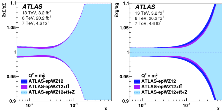
Figure 8. Impact of the ATLAS Z boson and t\bar{t} cross-section data on the determination of PDFs. The bands represent the uncertainty for the ATLAS-epWZ12 PDF set and the uncertainty of the profiled ATLAS-epWZ12 PDF set using Z boson and t\bar{t} data as a function of x for the total light-quark-sea distribution (left) for the gluon density (right). The plots also show the impact of only including the ATLAS t\bar{t} data set. Taken from Ref. [4].
