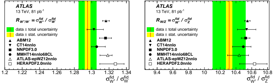
Figure 6. Ratios (red line) of W^+ to W^- boson (left) and W to Z boson (right) combined production cross sections in the fiducial region compared to predictions based on different PDF sets. The inner (yellow) shaded band corresponds to the statistical uncertainty while the outer (green) band shows statistical and systematic uncertainties added in quadrature. The theory predictions are given with only the corresponding PDF uncertainties shown as error bars. Taken from Ref. [3].
