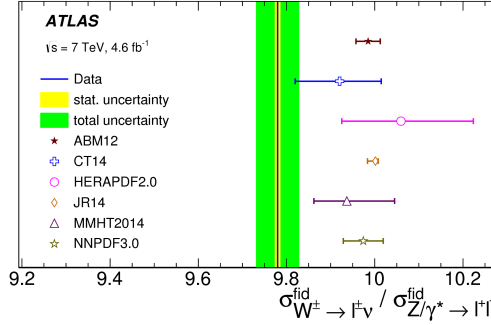
Figure 2. Fiducial cross sections times leptonic branching ratios of the W \rightarrow l\nu/Z \rightarrow ll ratio. The data (solid blue line) are shown with the statistical (yellow band) and the total uncertainties (green band). The uncertainties of the theoretical calculations correspond to the PDF uncertainties only. Taken from Ref. [2].
