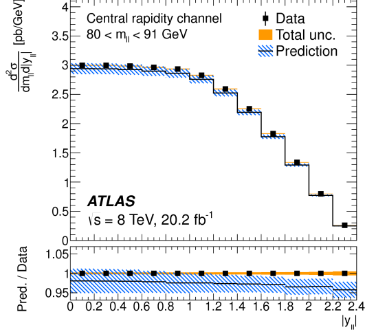
Figure 10. Fiducial cross section as a function of m_{\ell\ell} , the dilepton rapidity |y_{\ell\ell}| in the invariant mass range close to the Z boson mass. The data are shown as solid markers and the prediction from Powheg is shown as the solid line. The inner error bars represent the data statistical uncertainty and the solid band shows the total experimental uncertainty. The contribution to the uncertainty from the luminosity measurement is excluded. The hatched band represents the statistical and PDF uncertainties in the prediction. Taken from Ref. [6].
