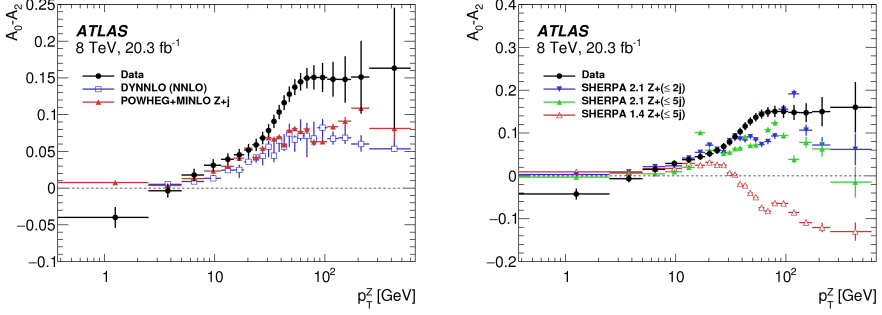
Figure 11. Distributions of the angular coefficients A_0 - A_2 as a function of p_T^Z . The results are compared to the DYNNLO and POWHEG MINLO predictions (left) and various SHERPA predictions (right). The error bars for the calculations show the total uncertainty for DYNNLO, but only the statistical uncertainties for POWHEG MINLO and SHERPA. Taken from Ref. [7].
