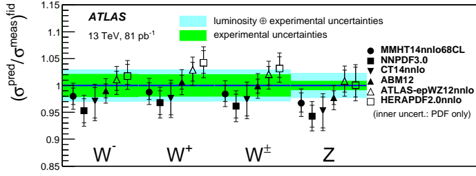
Figure 5. Ratio of the predicted to measured fiducial cross section for the combined electron and muon channels using various PDFs. The inner (outer) band corresponds to the experimental uncertainty without (with) the luminosity uncertainty. The inner error bar of the predictions represents the PDF uncertainty while the outer error bar includes the sum in quadrature of all other systematic uncertainties. Taken from Ref. [3].
