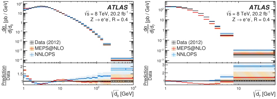
Figure 12. Charged-only distributions for the 0-th (left) and the 7-th (right) splitting scales in the electron channel using the jet-radius parameter R=0.4 . The size of the error bars reflects the statistical uncertainty, while the combined statistical and systematic uncertainty is indicated by the grey band. Theoretical predictions from SHERPA with NLO multijet merging (MEPS@NLO) and from POWHEG+PYTHIA8 with NNLO matching (NNLOPS) are displayed including error bands for the generator uncertainties. Taken from Ref. [8].
