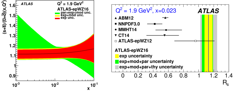
Figure 4. Left: R_s ratio of the PDFs from the present ATLAS-epWZ16 determination shown in the region of maximum sensitivity of the ATLAS data, 10^{-3} < x < 10^{-1} . Uncertainty bands represent the experimental (exp), model (mod) and parameterization (par) components in red, yellow and green, respectively. Right: R_s in the region of ATLAS best sensitivity, Q^2 = 1.9 \text{ GeV}^2 and x = 0.023 . Bands: present result and its uncertainty contributions from experimental data, QCD fit, and theoretical uncertainties; Closed symbols with horizontal error bars: predictions from different NNLO PDF sets; Open square: previous ATLAS results. Taken from Ref. [2].
