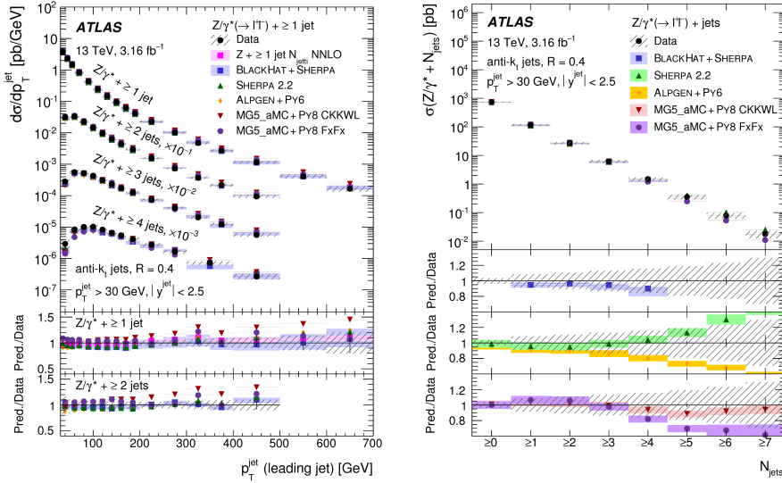
Figure 9. Left: measured cross section as a function of the leading jet p_T for inclusive Z + \geq 1, 2, 3, 4 jet events. Right: measured cross section as a function of the inclusive jet multiplicity for Z + \text{jets} events. The data are compared to the predictions from Z + \geq 1 jet N_{\text{jets}} NNLO ( p_T spectra only), BLACKHAT+SHERPA, SHERPA 2.2, ALPGEN+PY6, MG5_aMC+PY8 CKKWL, and MG5_aMC+PY8 FxFx. The error bars correspond to the statistical uncertainty, and the hatched bands to the data statistical and systematic uncertainties (including luminosity) added in quadrature. Taken from Ref. [5].
