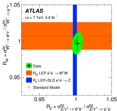
Figure 1. Measurement of the electron-to-muon cross-section ratios for the W and Z bosons. The green shaded ellipse represents the 68% CL for the correlated measurement of W and Z ratios, while the black error bars give the one-dimensional standard deviation. The orange and blue shaded bands represent the combination of the ratios as measured at the LEP and SLAC e^+e^- colliders. The SM expectation is indicated with an open circle. Taken from Ref. [2].
