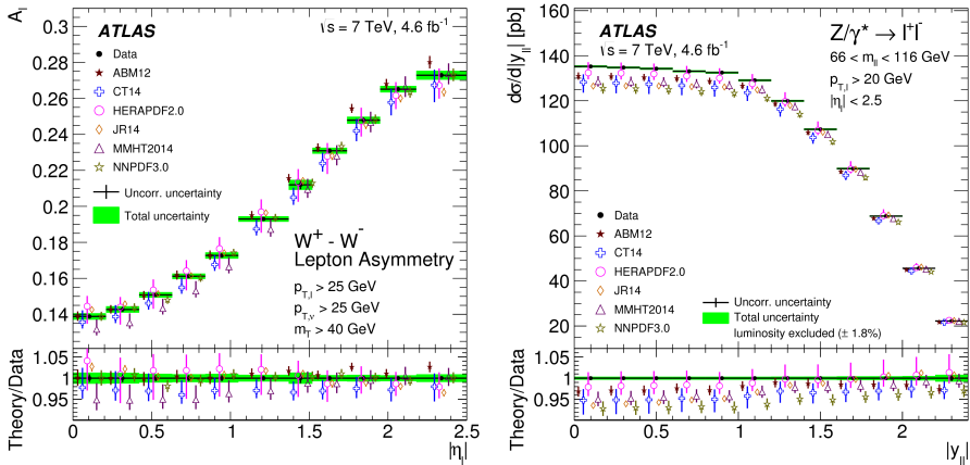
Figure 3. Left: lepton charge asymmetry A_l production as a function of the lepton pseudorapidity. Right: Z boson differential cross-section measurement as a function of the leptons rapidity |y_{ll}| . Predictions computed at NNLO QCD with NLO EW corrections using various PDF sets (open symbols) are compared to the data (full points). The ratio of theoretical predictions to the data is also shown. The predictions are displaced within each bin for better visibility. The theory uncertainty corresponds to the quadratic sum of the PDF uncertainty and the statistical uncertainty of the calculation. Taken from Ref. [2].
